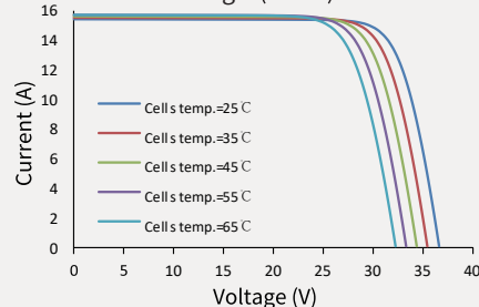
Current-Voltage (460W)
